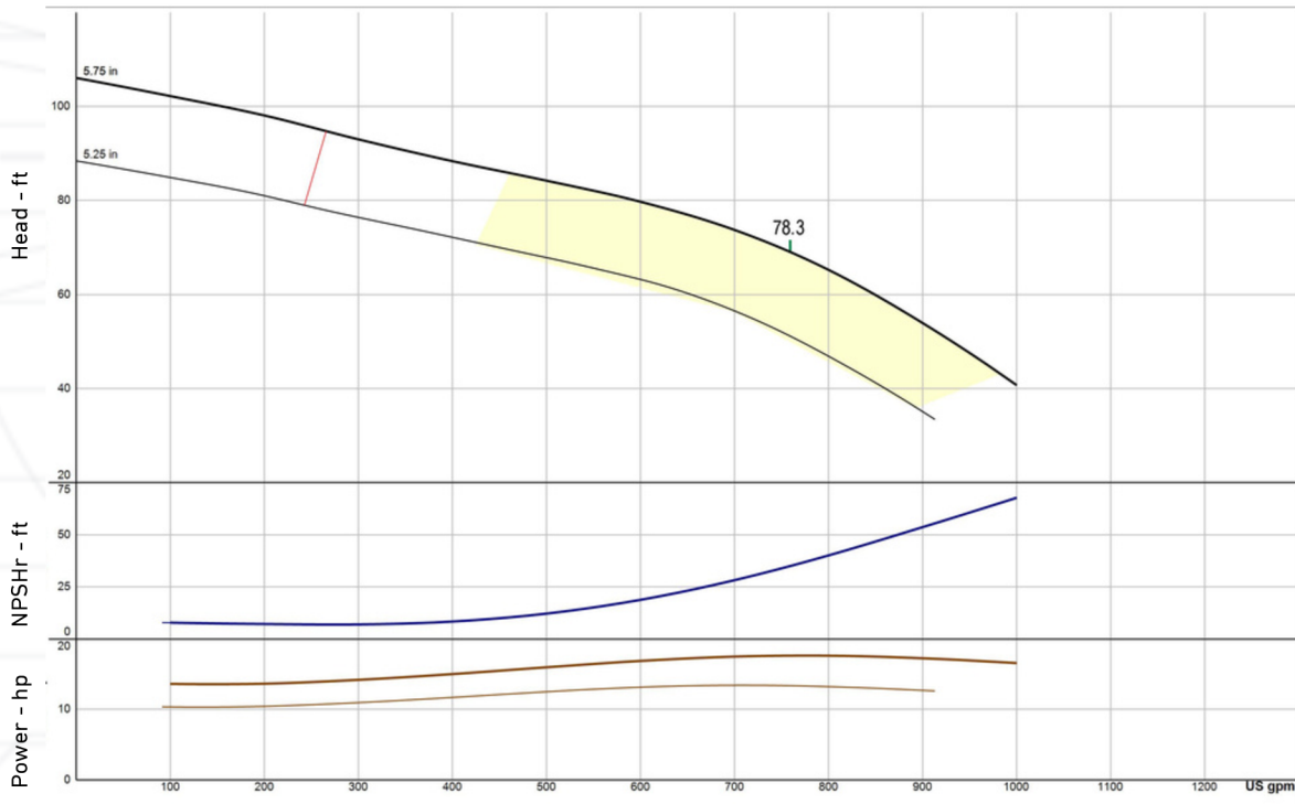
SM7M 3450RPM 2-POLE SPEED PERFORMANCE CURVE
